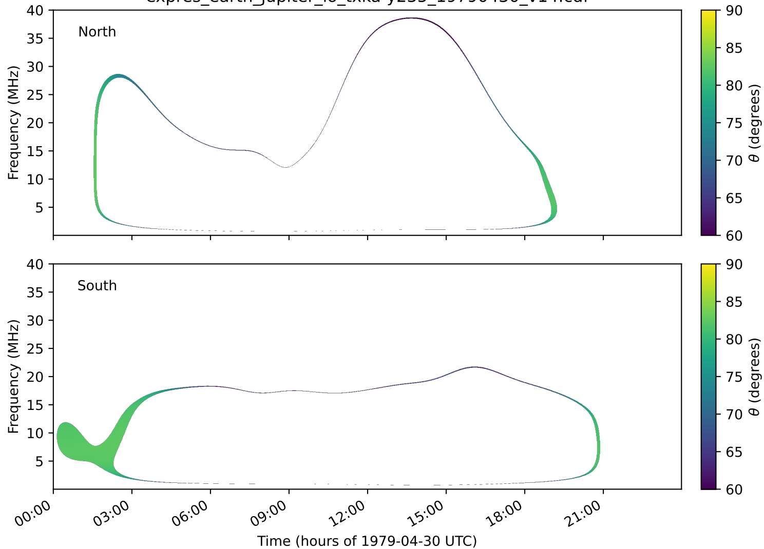
expres_earth_jupiter_io_txka-y235_19790430_v14.cdf
