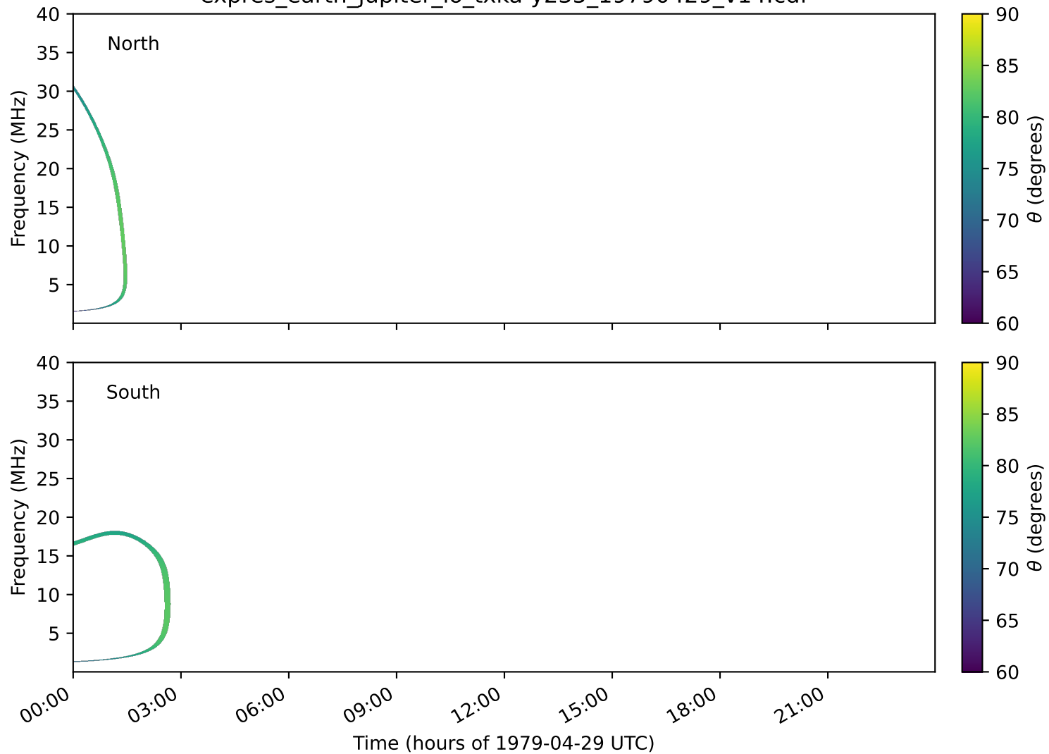
expres_earth_jupiter_io_txka-y235_19790429_v14.cdf
