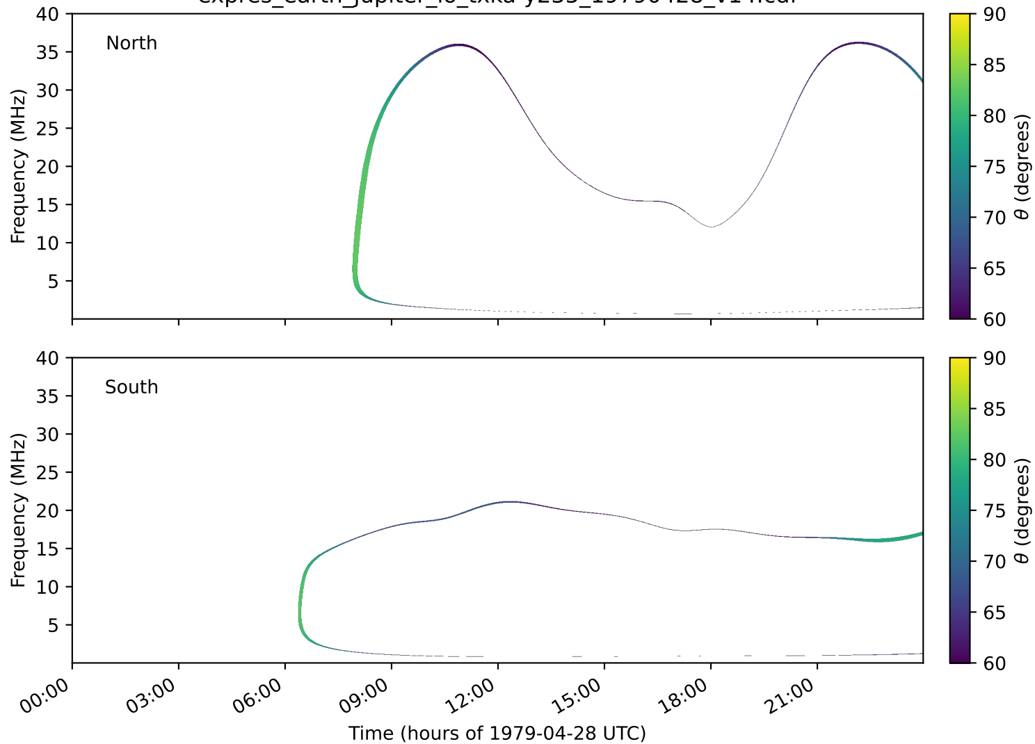
expres_earth_jupiter_io_txka-y235_19790428_v14.cdf
