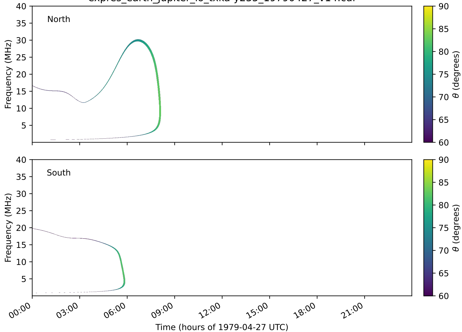
expres_earth_jupiter_io_txka-y235_19790427_v14.cdf
