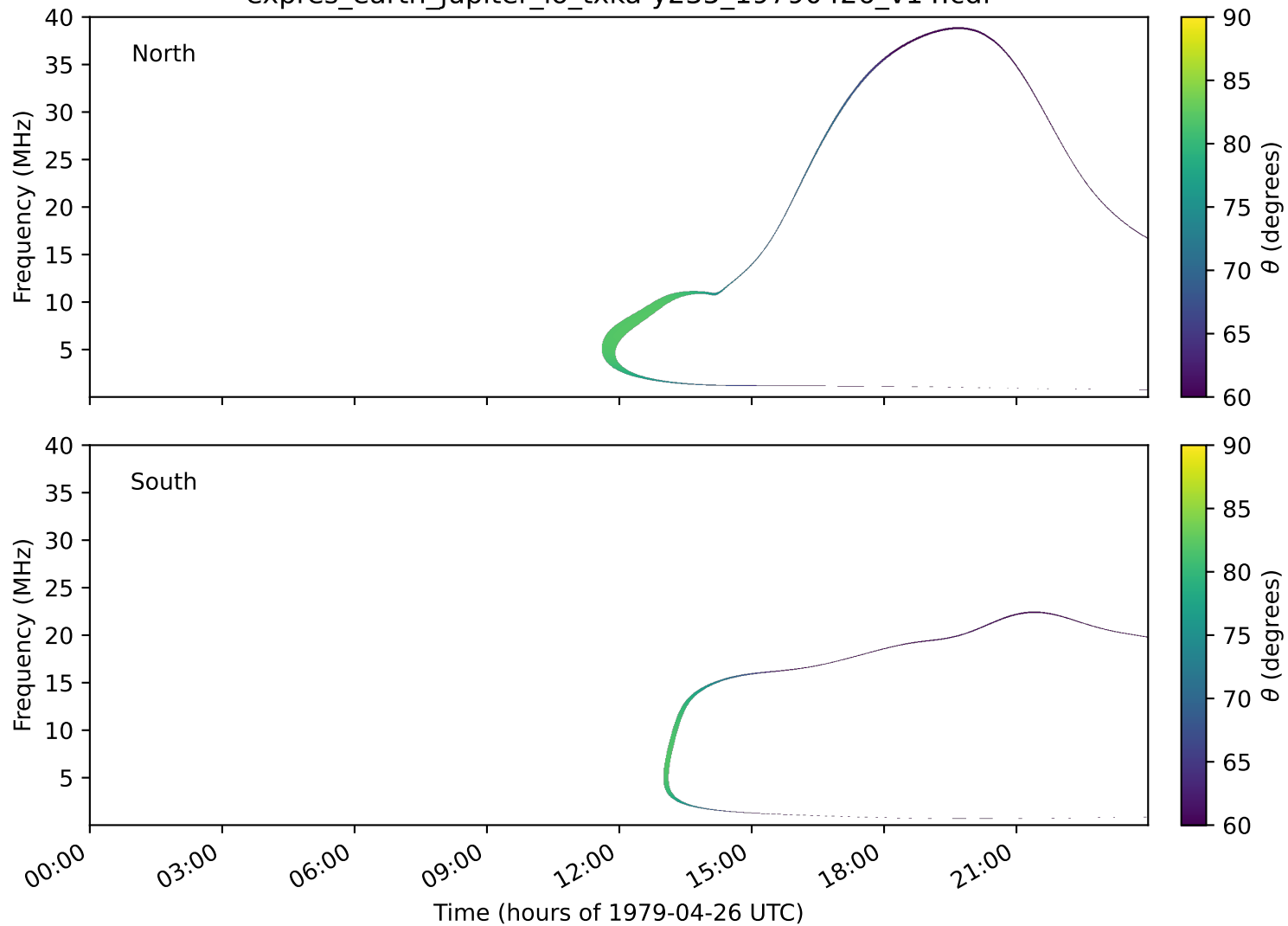
expres_earth_jupiter_io_txka-y235_19790426_v14.cdf
