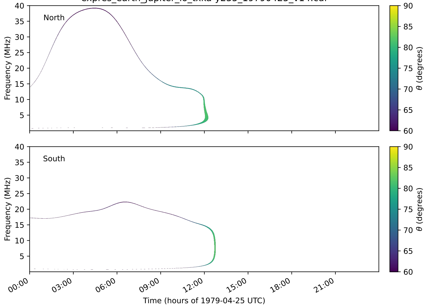
expres_earth_jupiter_io_txka-y235_19790425_v14.cdf
