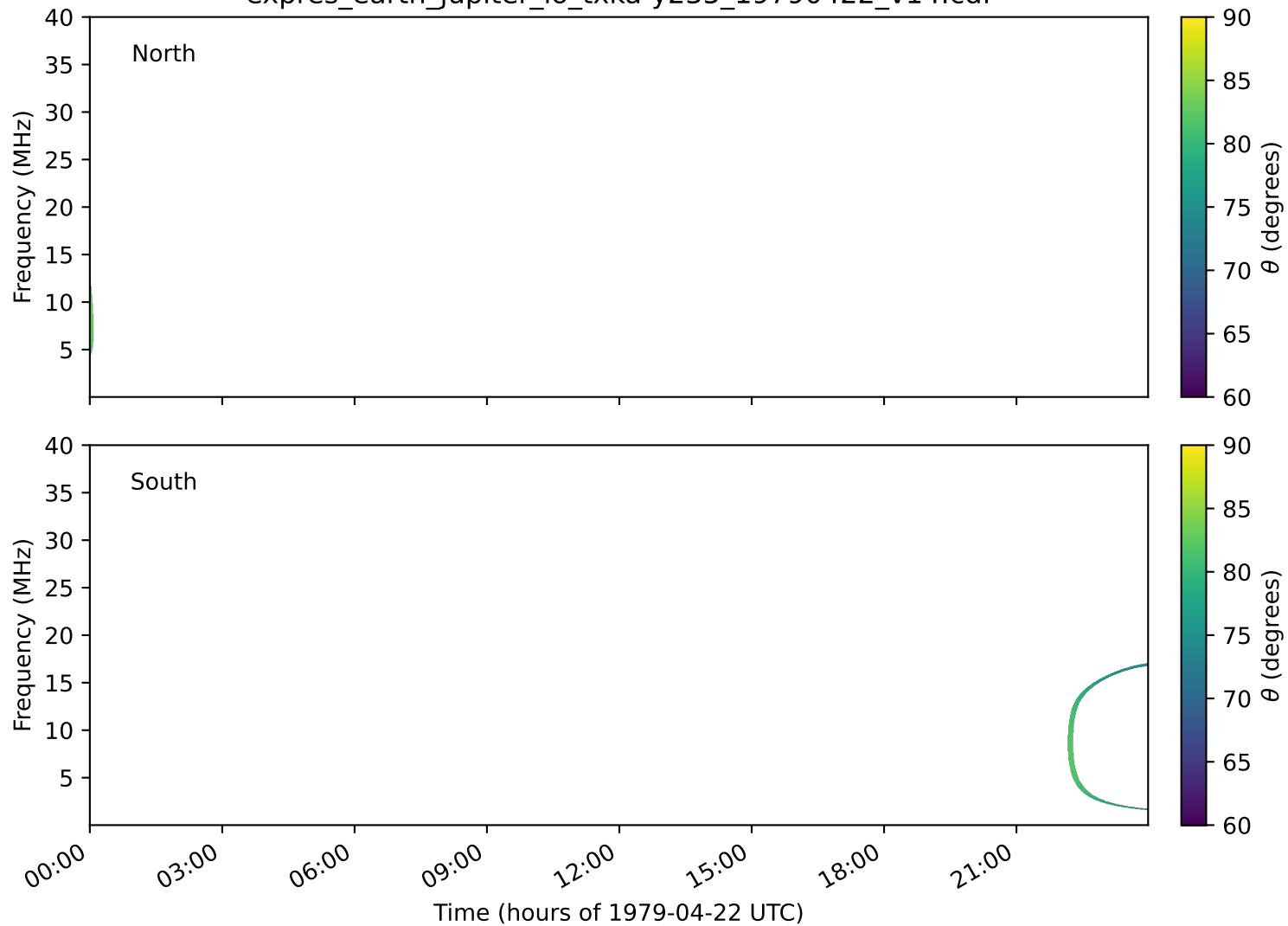
expres_earth_jupiter_io_txka-y235_19790422_v14.cdf
