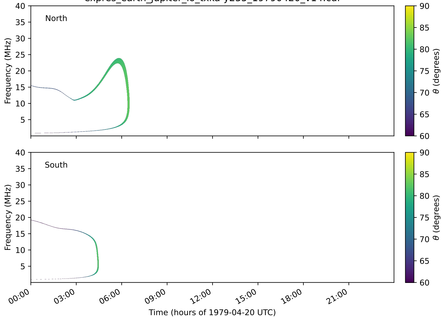
expres_earth_jupiter_io_txka-y235_19790420_v14.cdf
