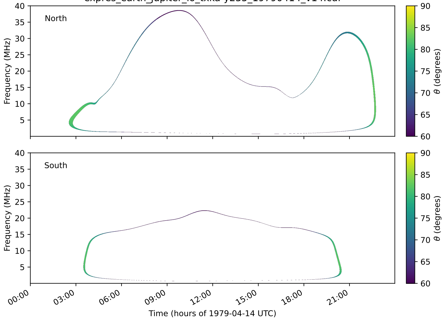
expres_earth_jupiter_io_txka-y235_19790414_v14.cdf
