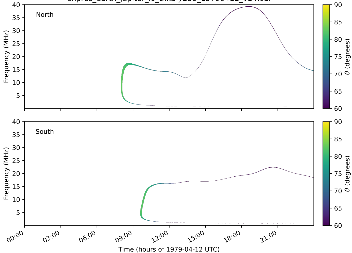
expres_earth_jupiter_io_txka-y235_19790412_v14.cdf
