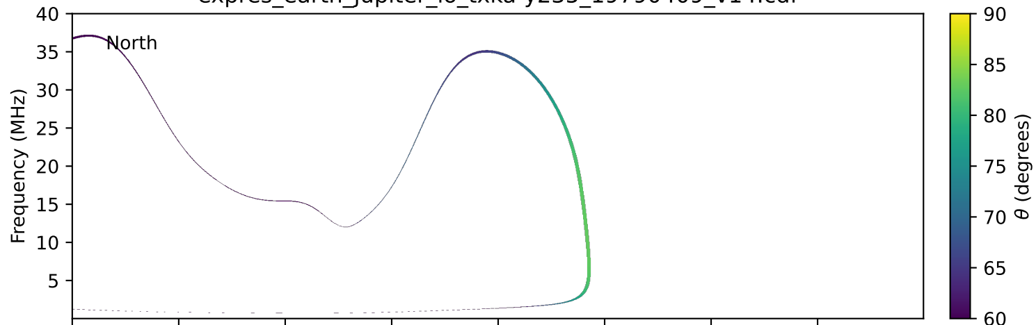
expres_earth_jupiter_io_txka-y235_19790409_v14.cdf
