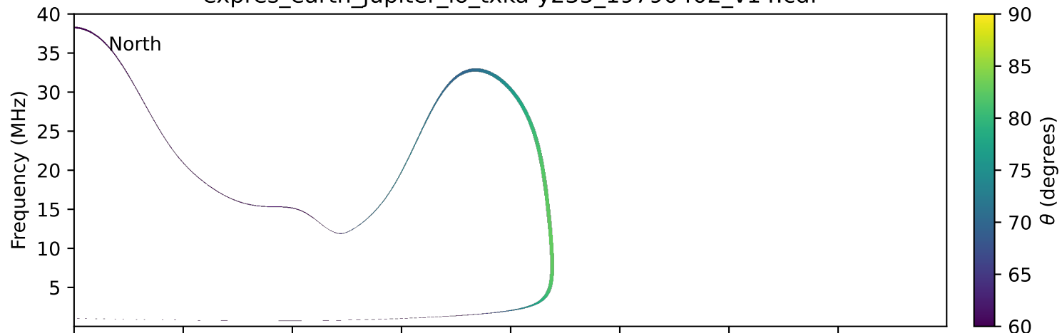
expres_earth_jupiter_io_txka-y235_19790402_v14.cdf
