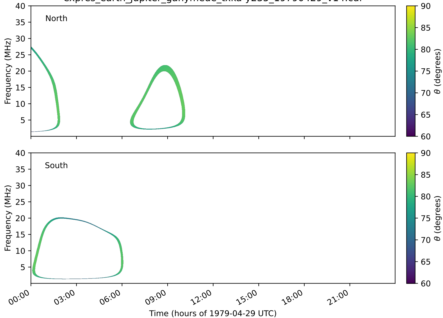
expres_earth_jupiter_ganymede_txka-y235_19790429_v14.cdf
