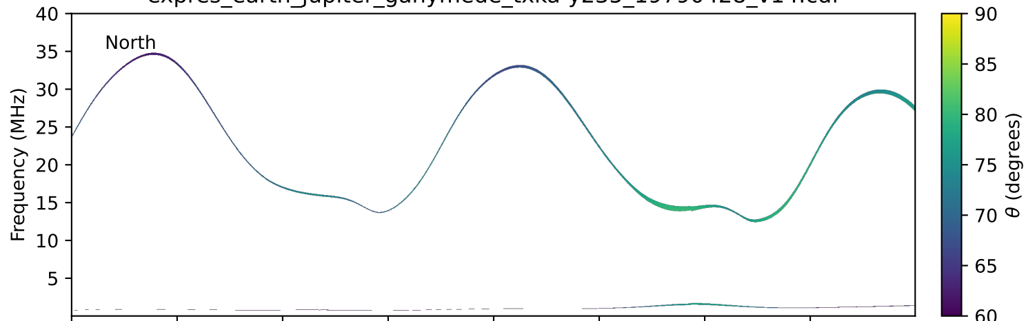
expres_earth_jupiter_ganymede_txka-y235_19790428_v14.cdf
