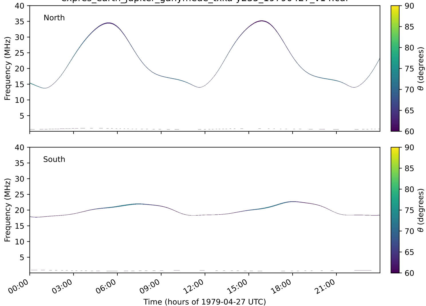
expres_earth_jupiter_ganymede_txka-y235_19790427_v14.cdf
