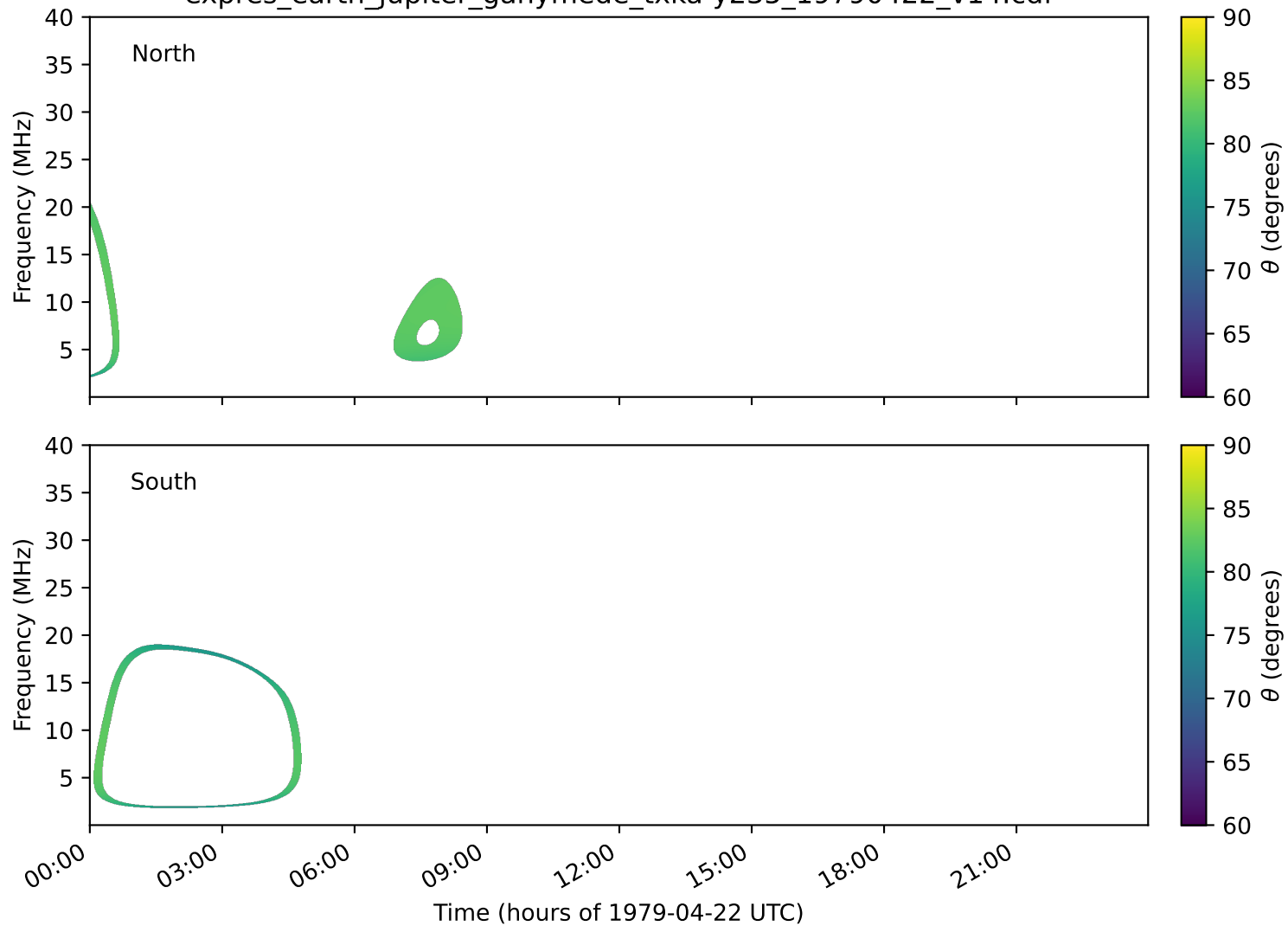
expres_earth_jupiter_ganymede_txka-y235_19790422_v14.cdf
