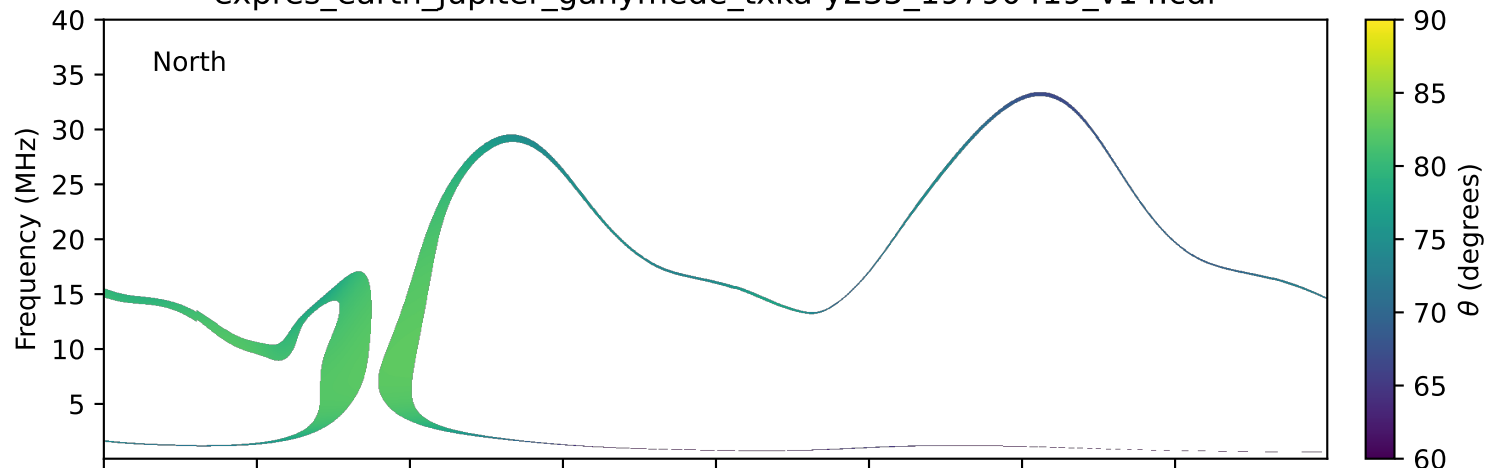
expres_earth_jupiter_ganymede_txka-y235_19790419_v14.cdf
