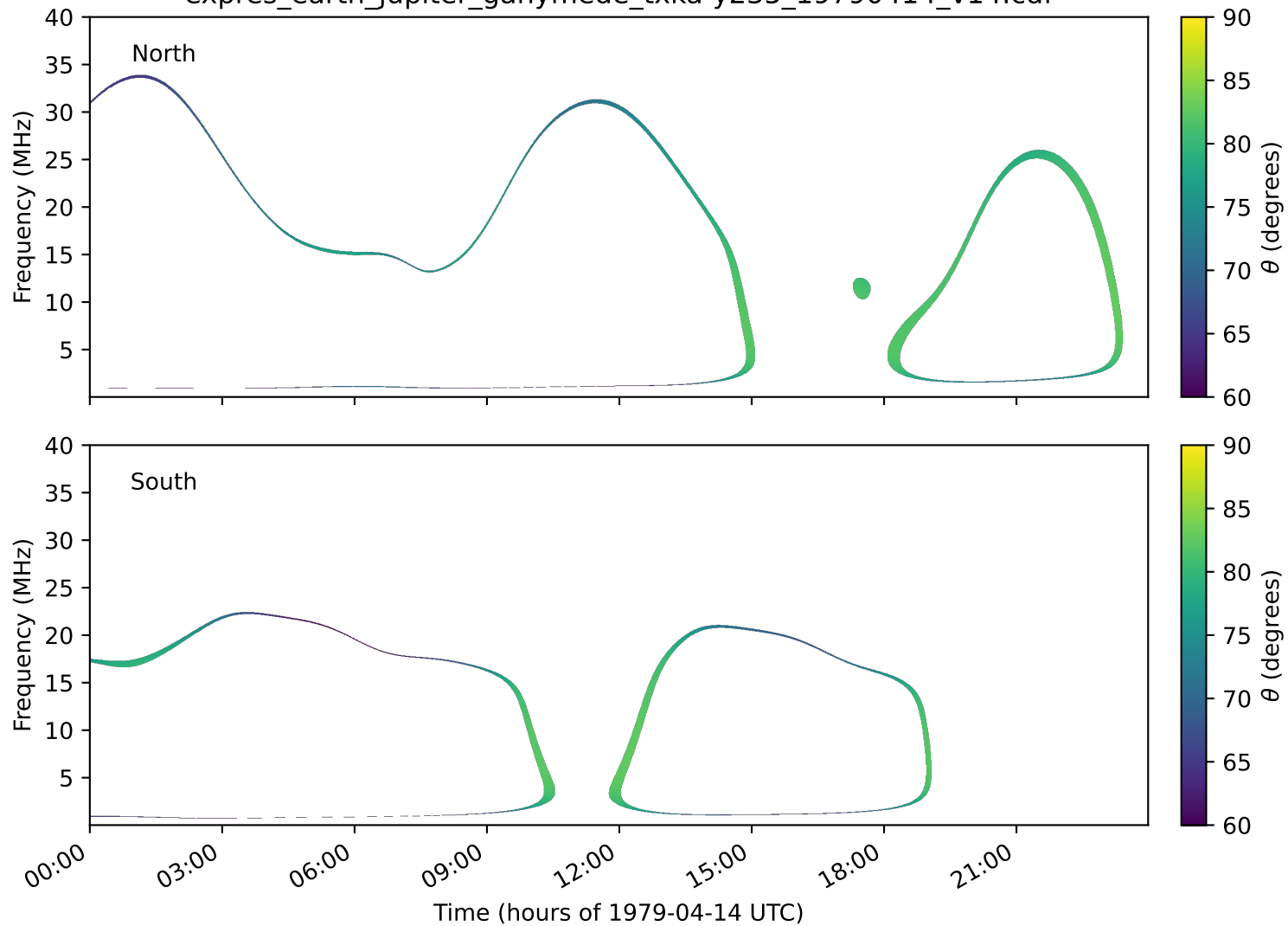
expres_earth_jupiter_ganymede_txka-y235_19790414_v14.cdf
