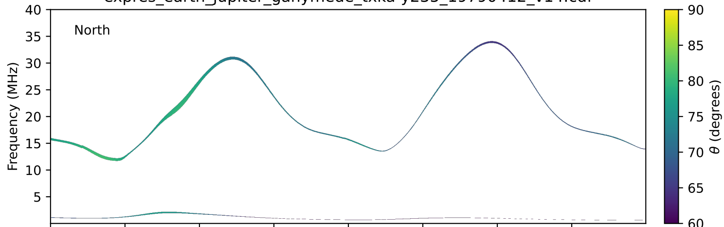
expres_earth_jupiter_ganymede_txka-y235_19790412_v14.cdf
