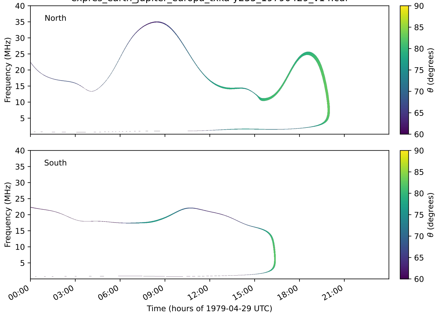
expres_earth_jupiter_europa_txka-y235_19790429_v14.cdf
