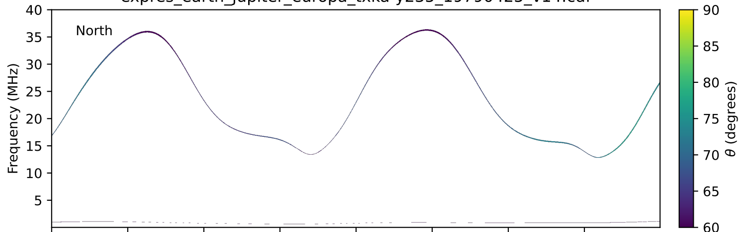
expres_earth_jupiter_europa_txka-y235_19790425_v14.cdf
