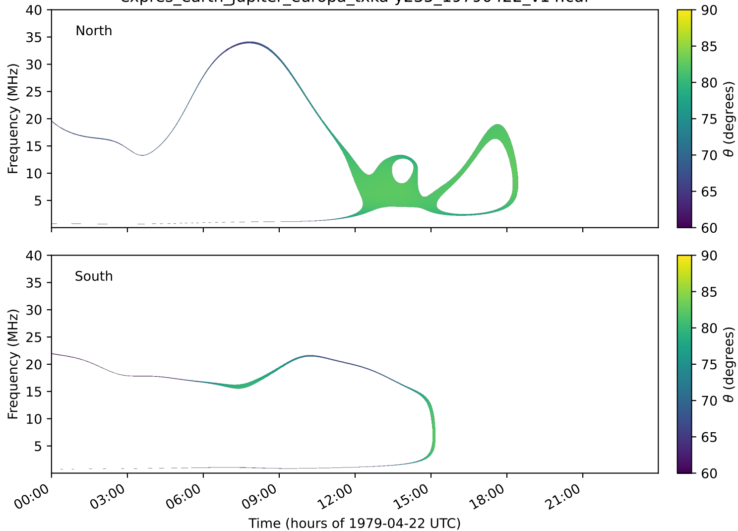
expres_earth_jupiter_europa_txka-y235_19790422_v14.cdf
