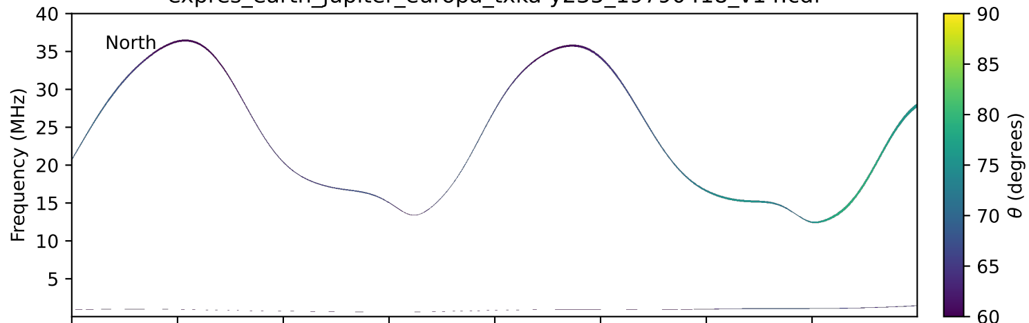
expres_earth_jupiter_europa_txka-y235_19790418_v14.cdf
