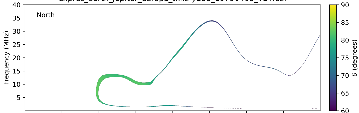
expres_earth_jupiter_europa_txka-y235_19790403_v14.cdf
