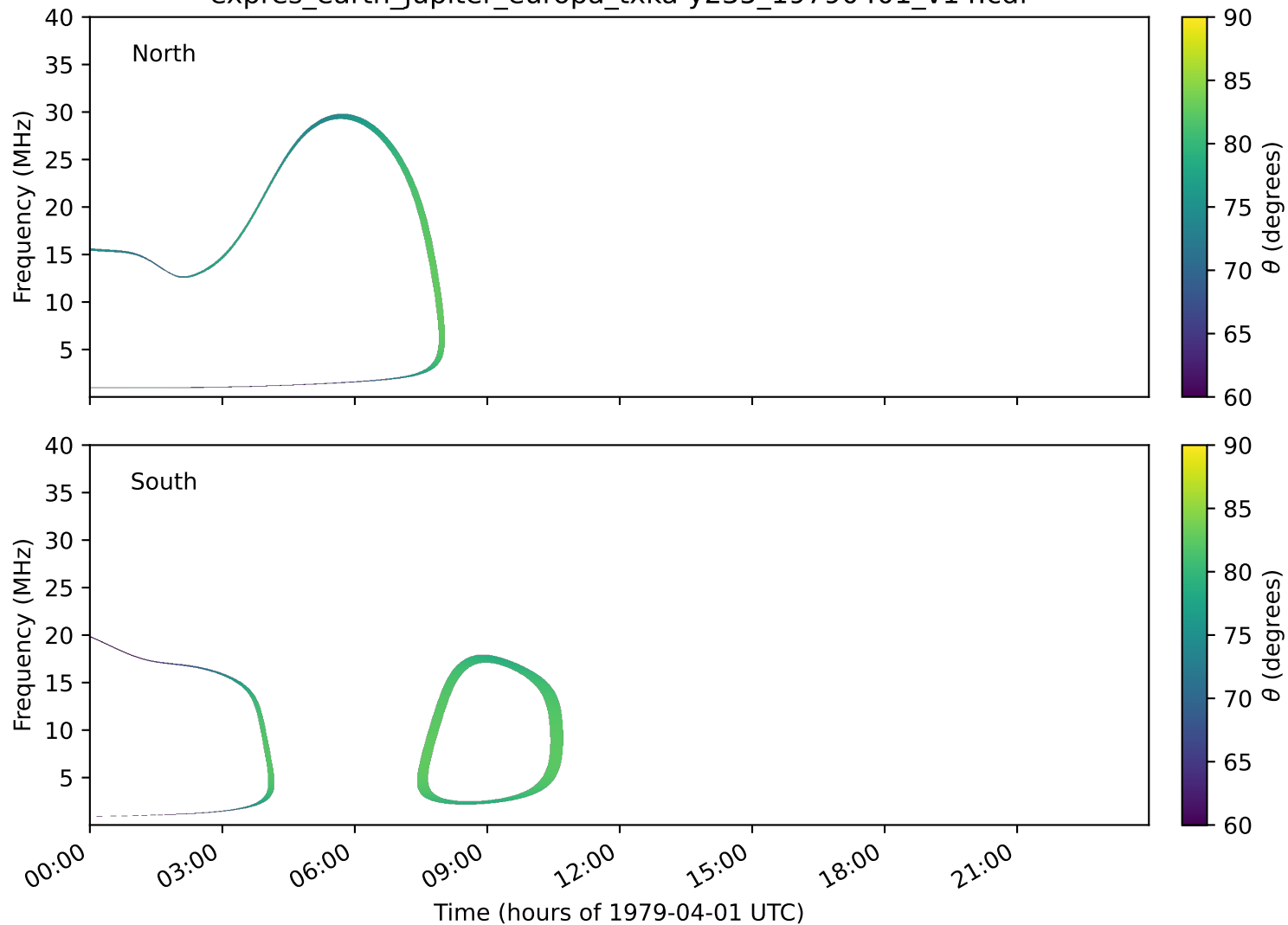
expres_earth_jupiter_europa_txka-y235_19790401_v14.cdf
