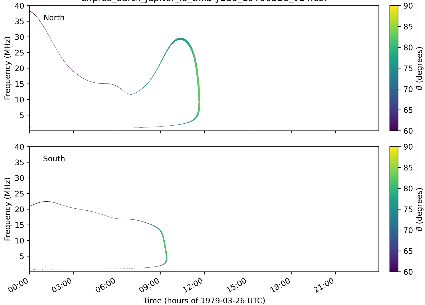
expres_earth_jupiter_io_txka-y235_19790326_v14.cdf
