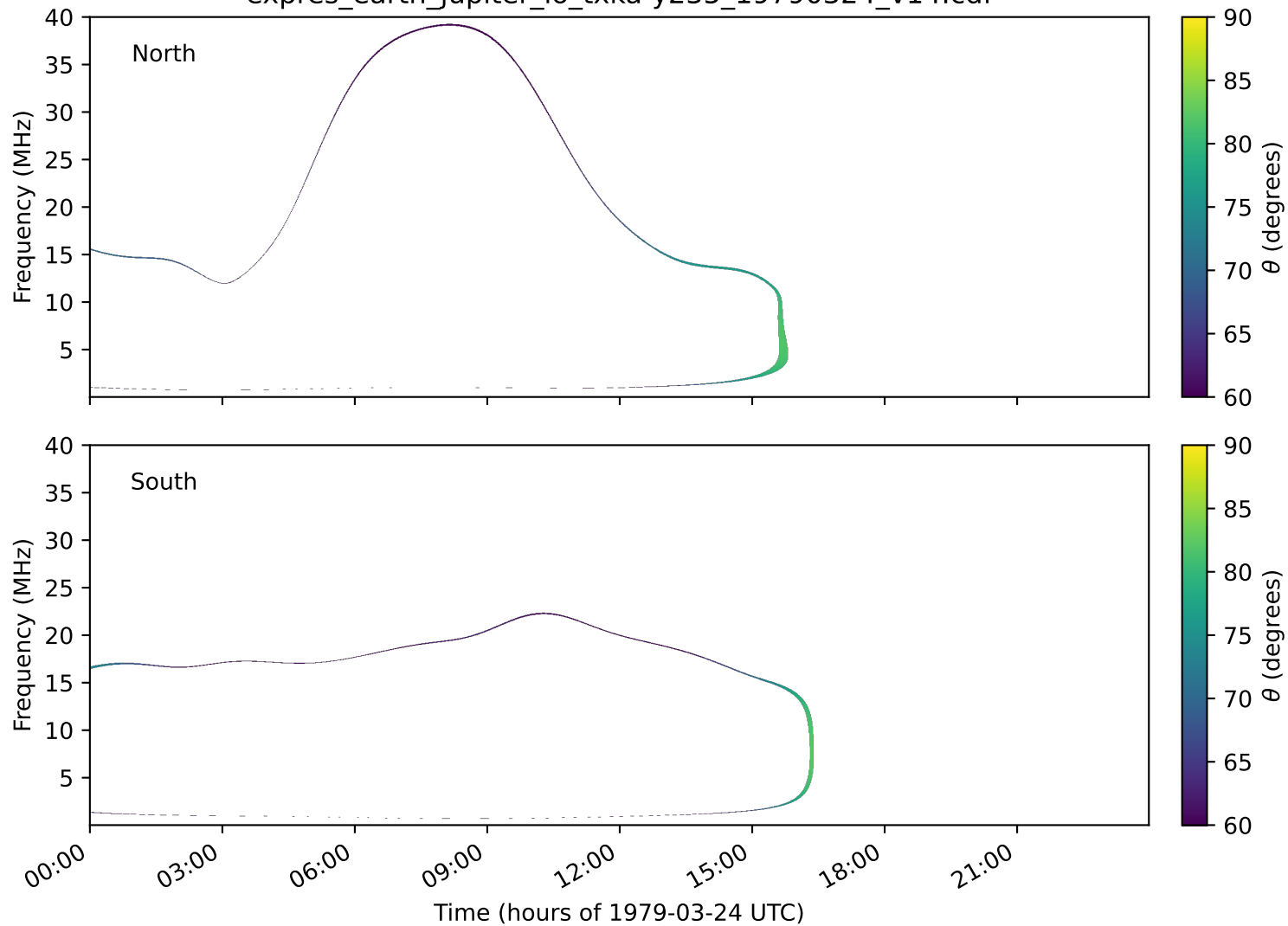
expres_earth_jupiter_io_txka-y235_19790324_v14.cdf
