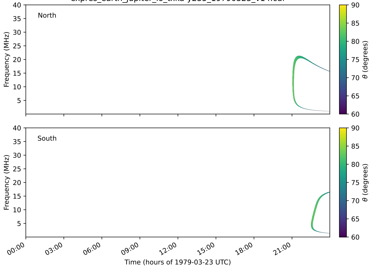
expres_earth_jupiter_io_txka-y235_19790323_v14.cdf
