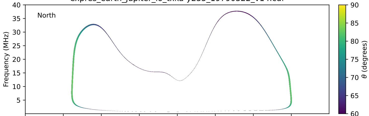
expres_earth_jupiter_io_txka-y235_19790322_v14.cdf
