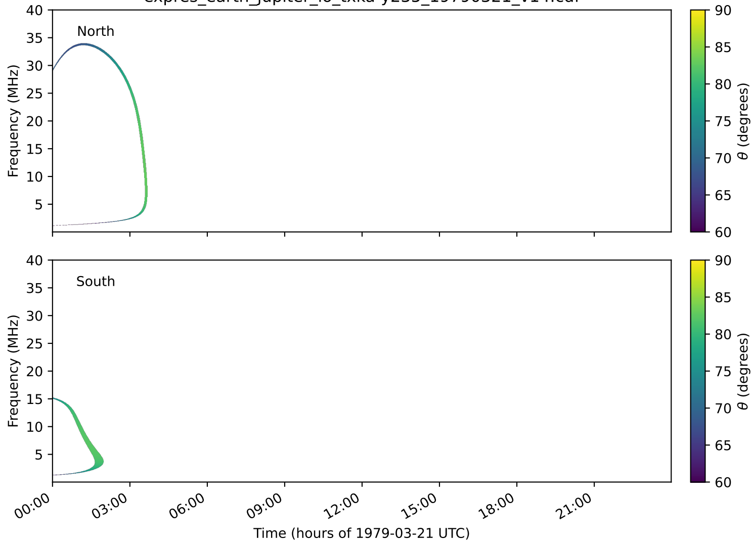
expres_earth_jupiter_io_txka-y235_19790321_v14.cdf
