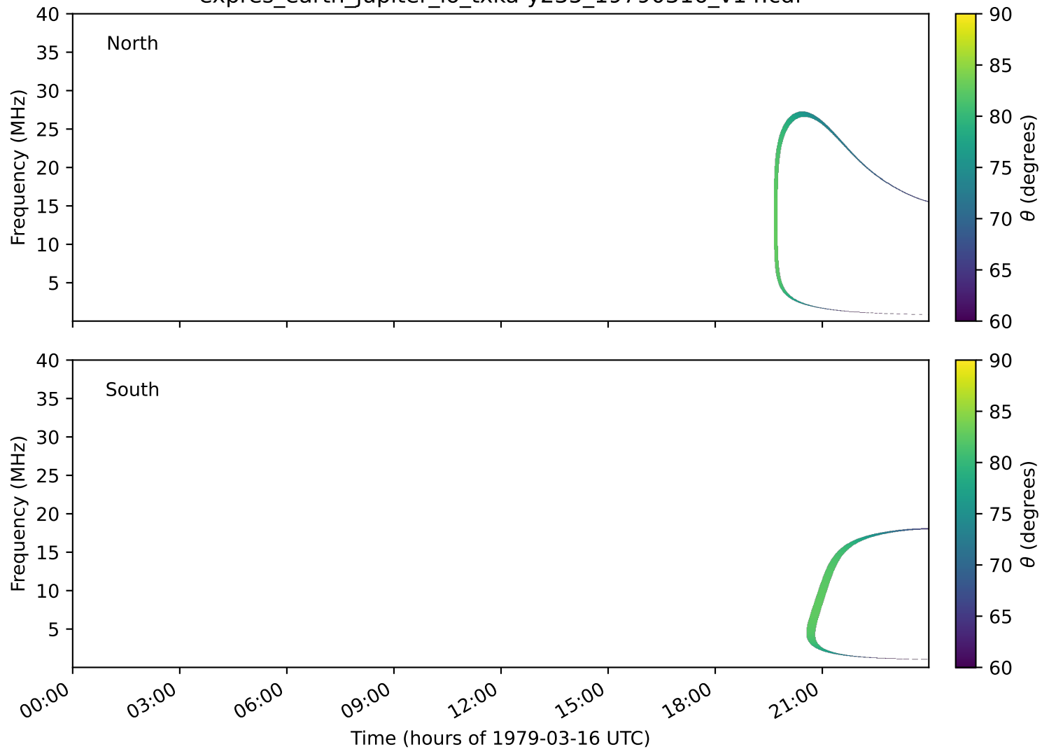
expres_earth_jupiter_io_txka-y235_19790316_v14.cdf
