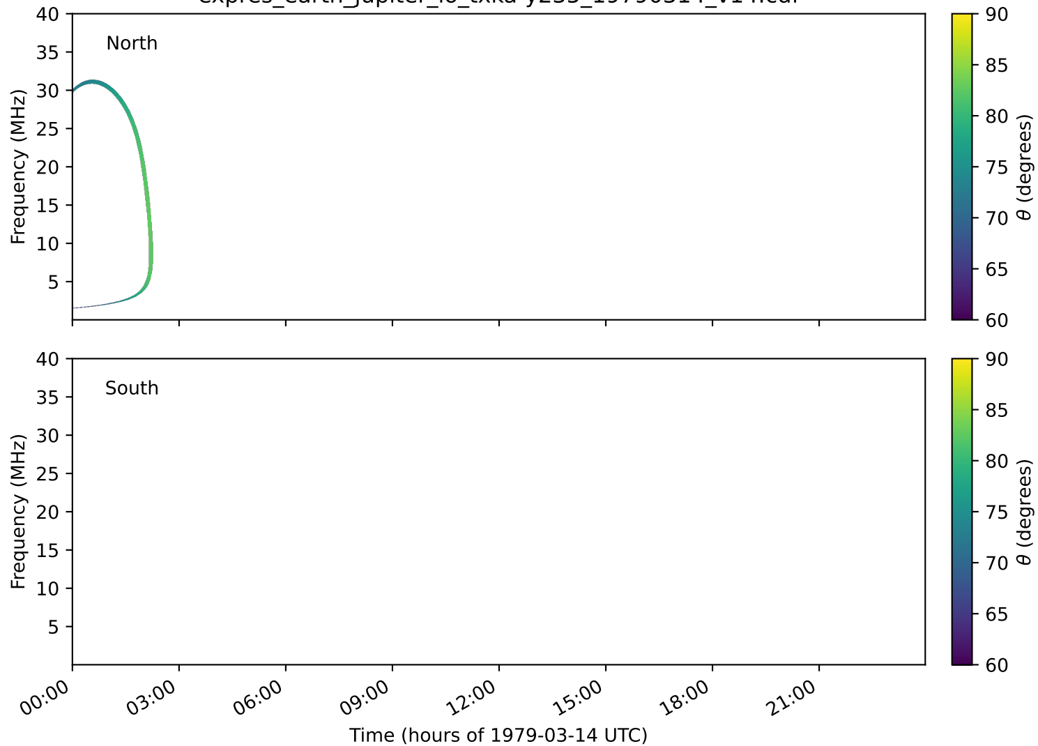
expres_earth_jupiter_io_txka-y235_19790314_v14.cdf
