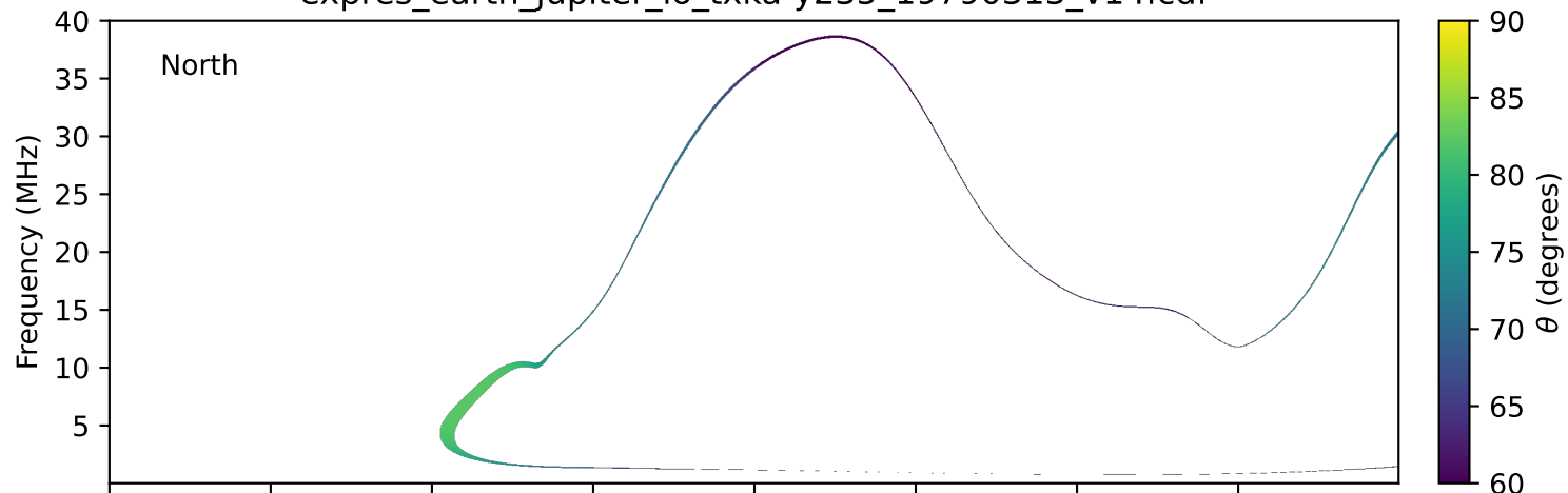
expres_earth_jupiter_io_txka-y235_19790313_v14.cdf
