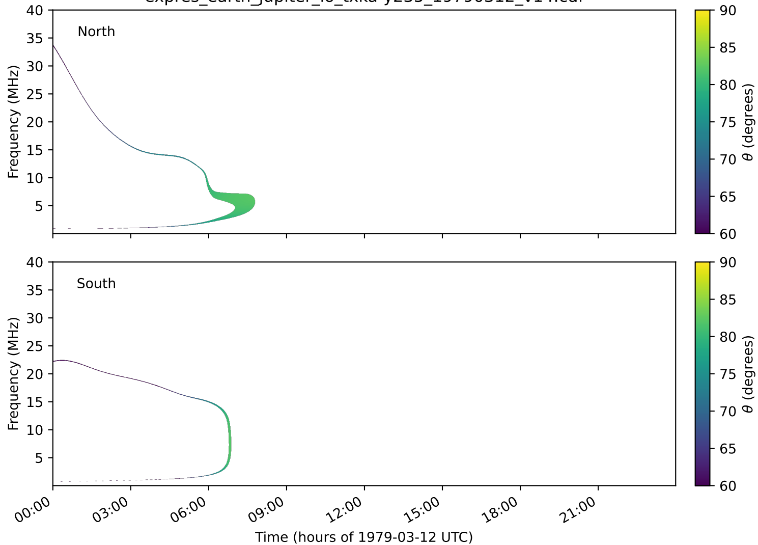
expres_earth_jupiter_io_txka-y235_19790312_v14.cdf
