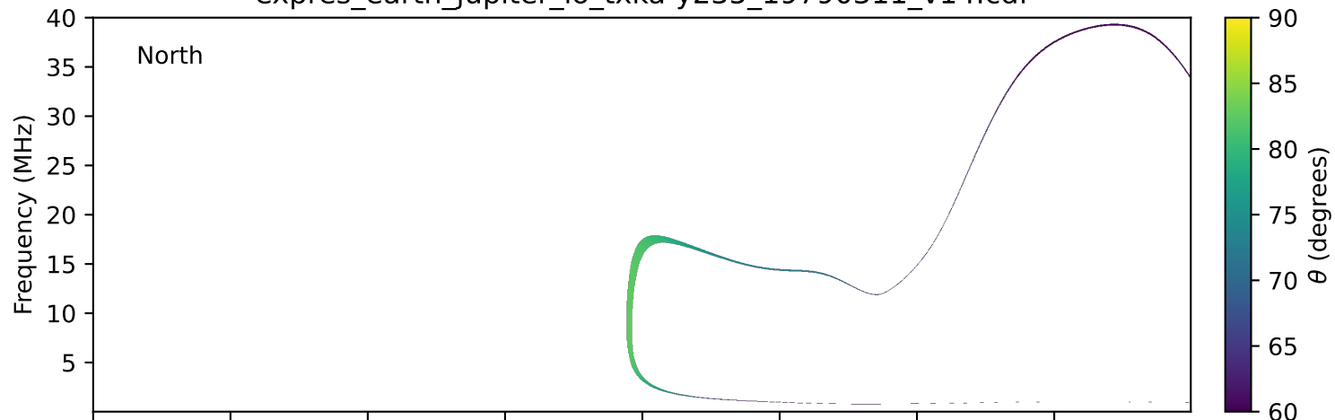
expres_earth_jupiter_io_txka-y235_19790311_v14.cdf
