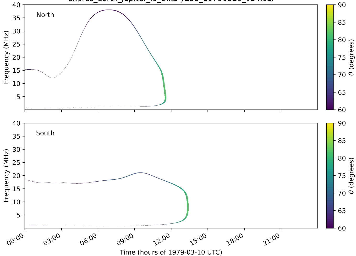
expres_earth_jupiter_io_txka-y235_19790310_v14.cdf
