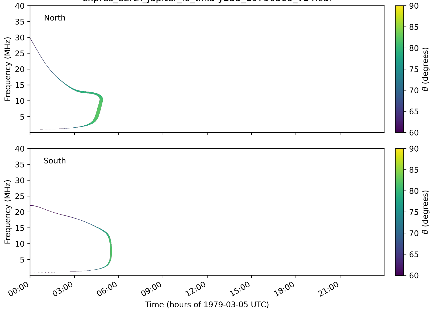
expres_earth_jupiter_io_txka-y235_19790305_v14.cdf
