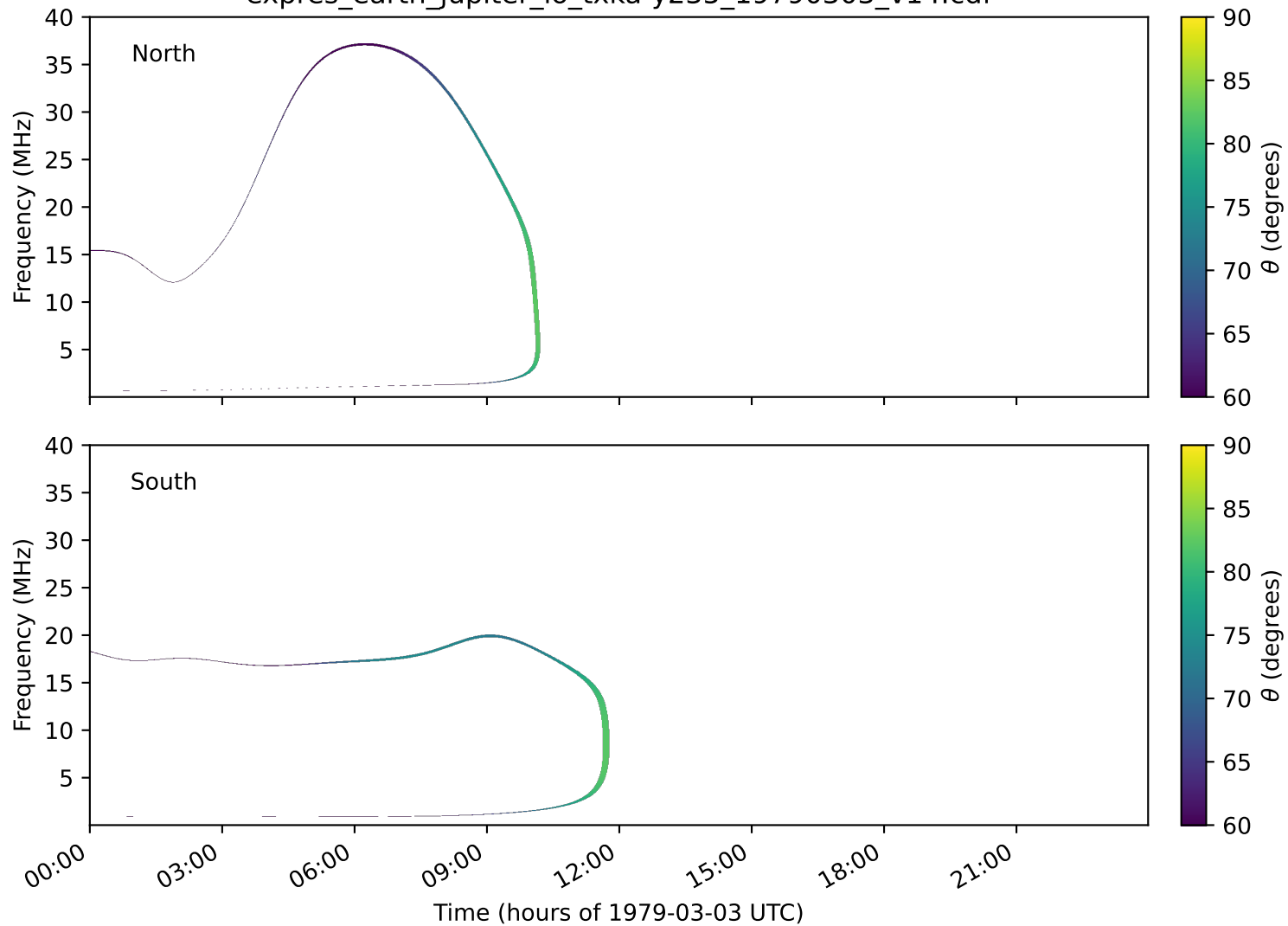
expres_earth_jupiter_io_txka-y235_19790303_v14.cdf
