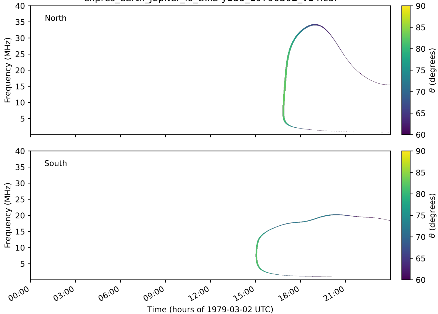
expres_earth_jupiter_io_txka-y235_19790302_v14.cdf
