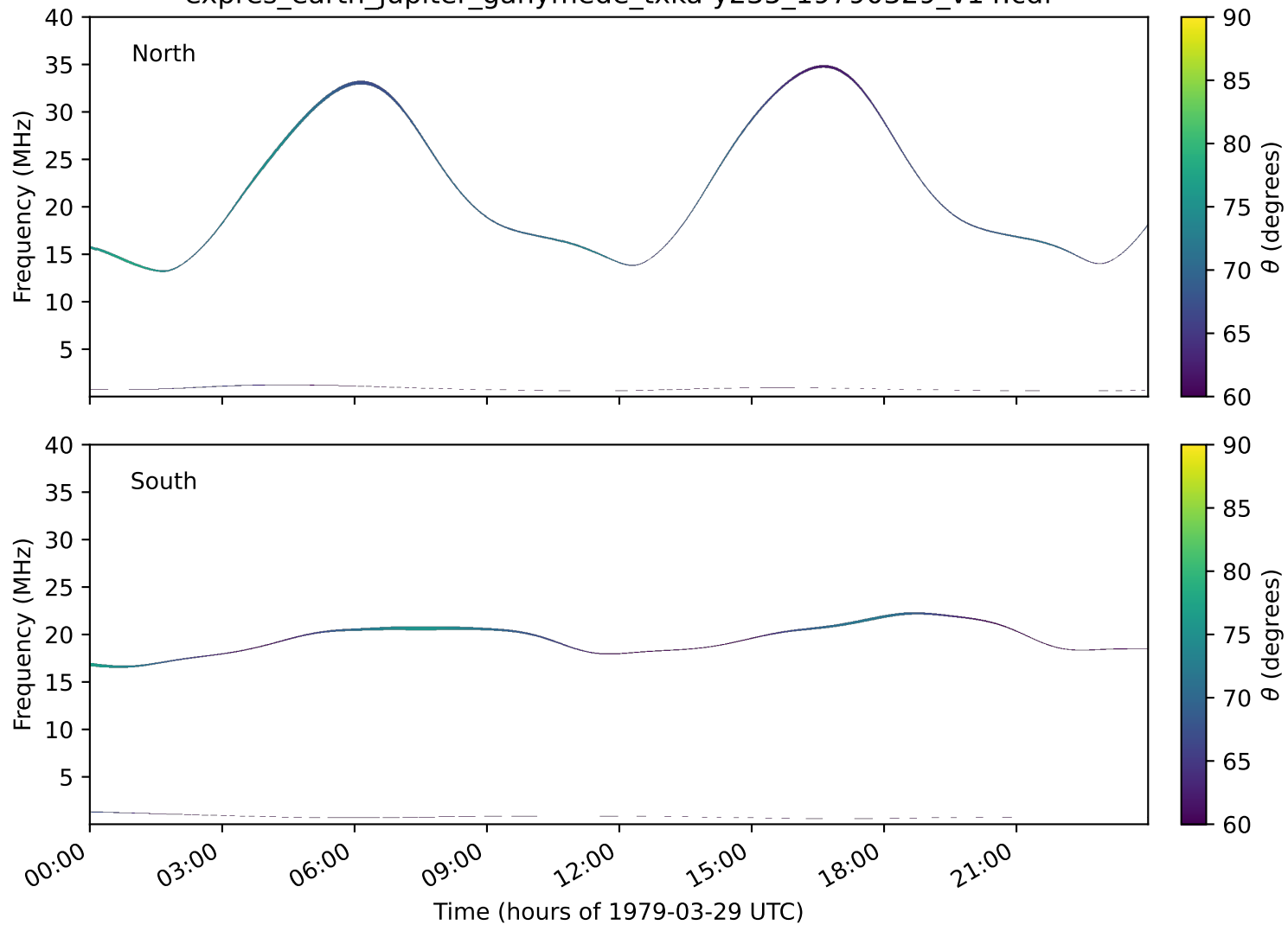
expres_earth_jupiter_ganymede_txka-y235_19790329_v14.cdf
