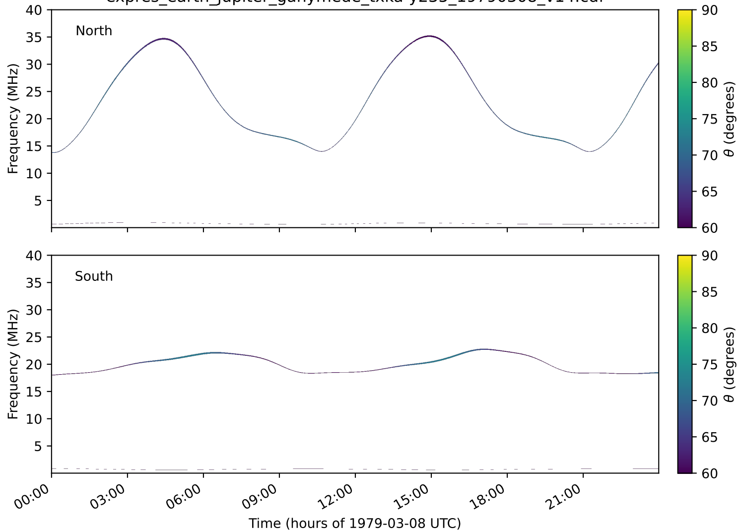
expres_earth_jupiter_ganymede_txka-y235_19790308_v14.cdf
