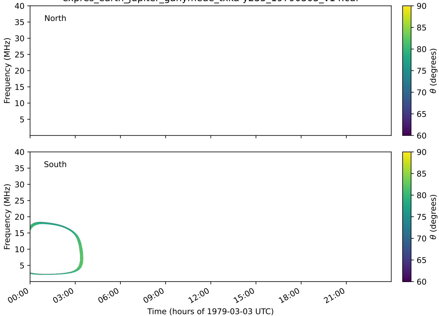
expres_earth_jupiter_ganymede_txka-y235_19790303_v14.cdf
