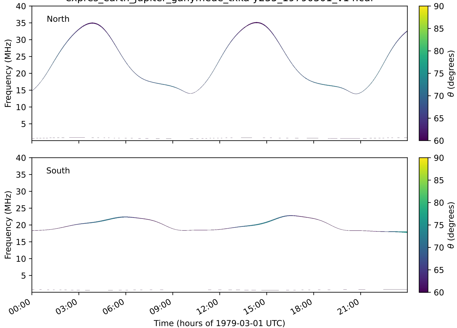
expres_earth_jupiter_ganymede_txka-y235_19790301_v14.cdf
