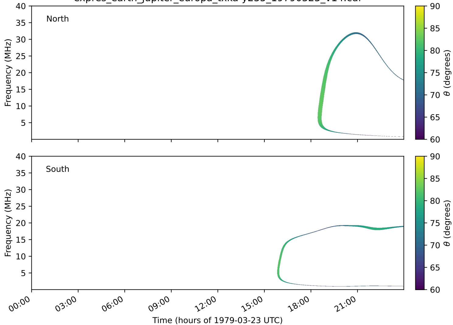
expres_earth_jupiter_europa_txka-y235_19790323_v14.cdf
