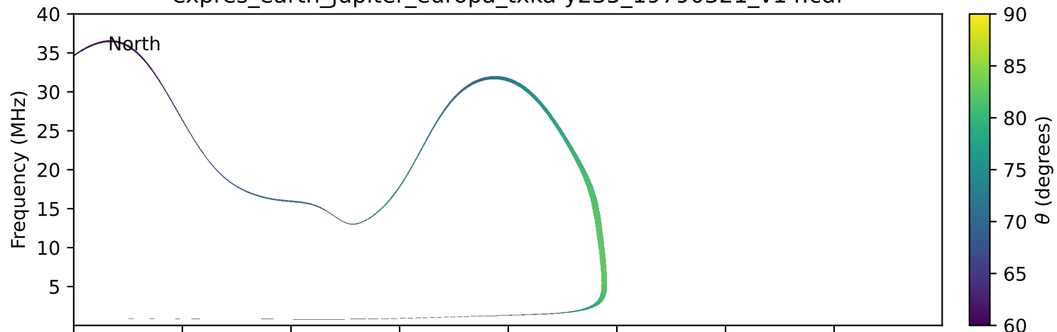
expres_earth_jupiter_europa_txka-y235_19790321_v14.cdf
