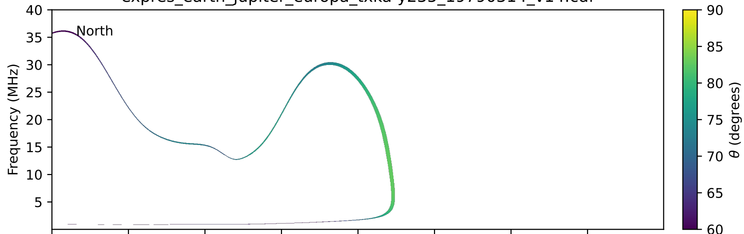
expres_earth_jupiter_europa_txka-y235_19790314_v14.cdf
