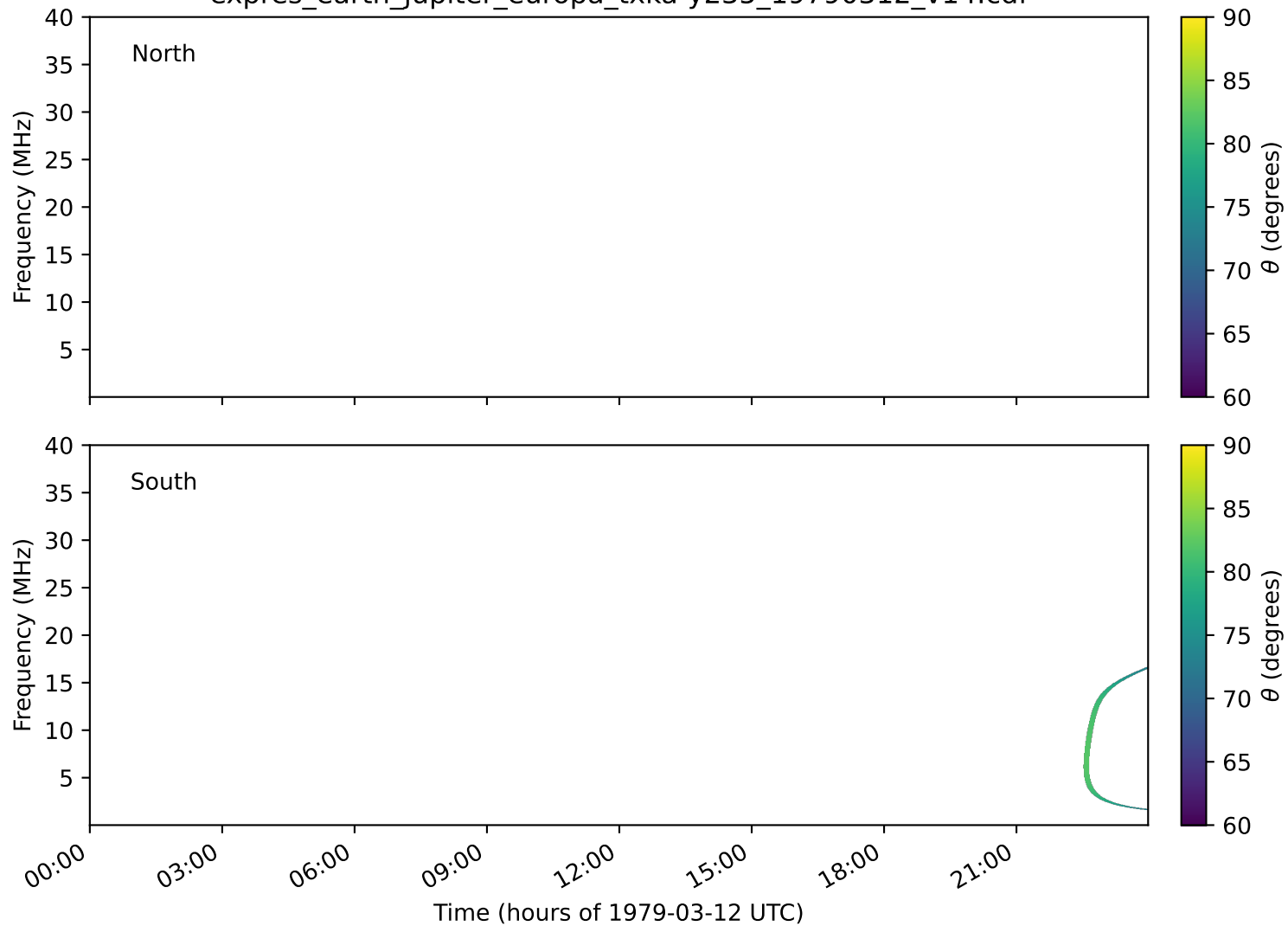
expres_earth_jupiter_europa_txka-y235_19790312_v14.cdf
