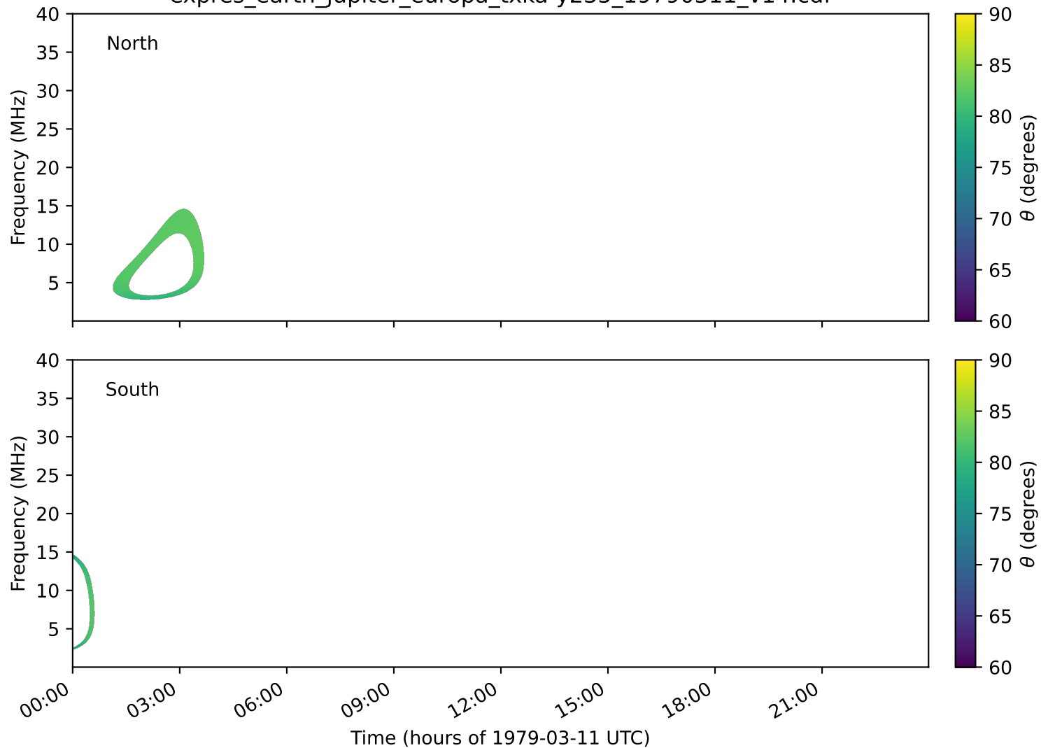
expres_earth_jupiter_europa_txka-y235_19790311_v14.cdf
