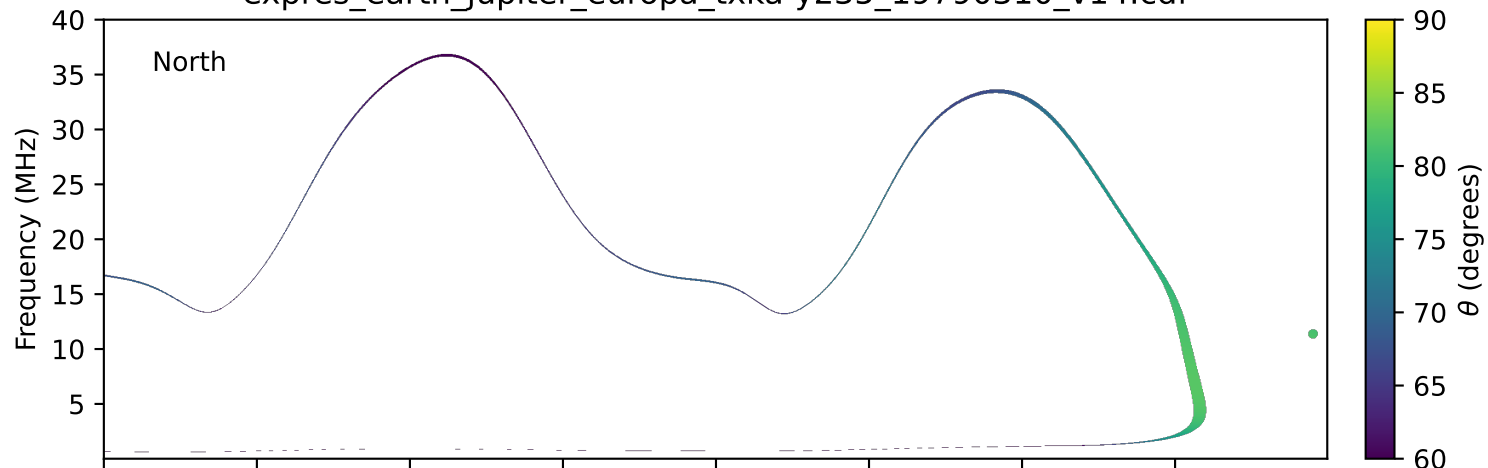
expres_earth_jupiter_europa_txka-y235_19790310_v14.cdf
