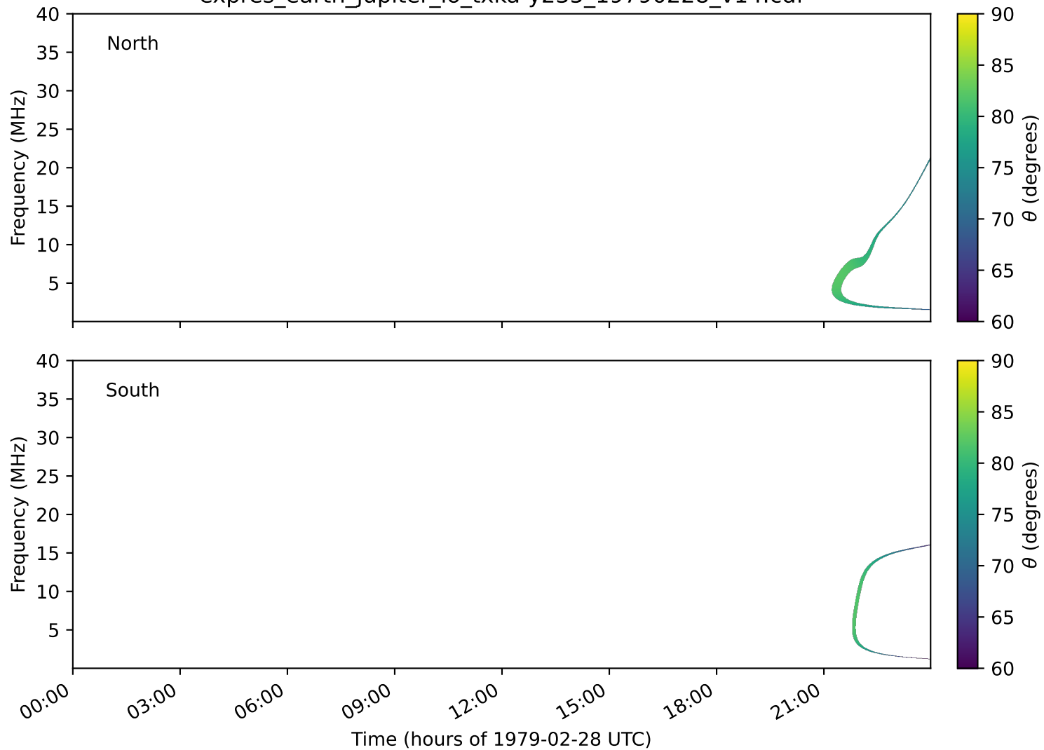
expres_earth_jupiter_io_txka-y235_19790228_v14.cdf
